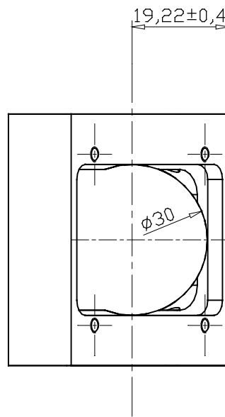
view B
