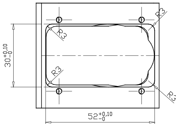
view A
